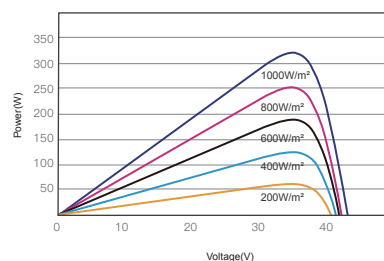
P-V CURVES OF PV MODULE(320W)
