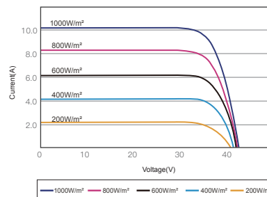
I-V CURVES OF PV MODULE(320W)
