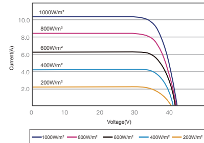
I-V CURVES OF PV MODULE(325W)
