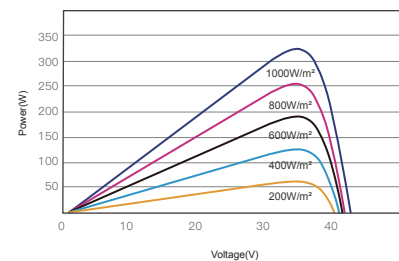
P-V CURVES OF PV MODULE(325W)
